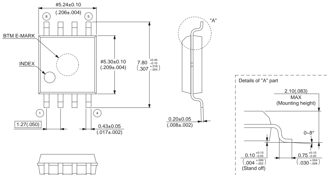
8-pin plastic SOP (FPT-8P-M08)
