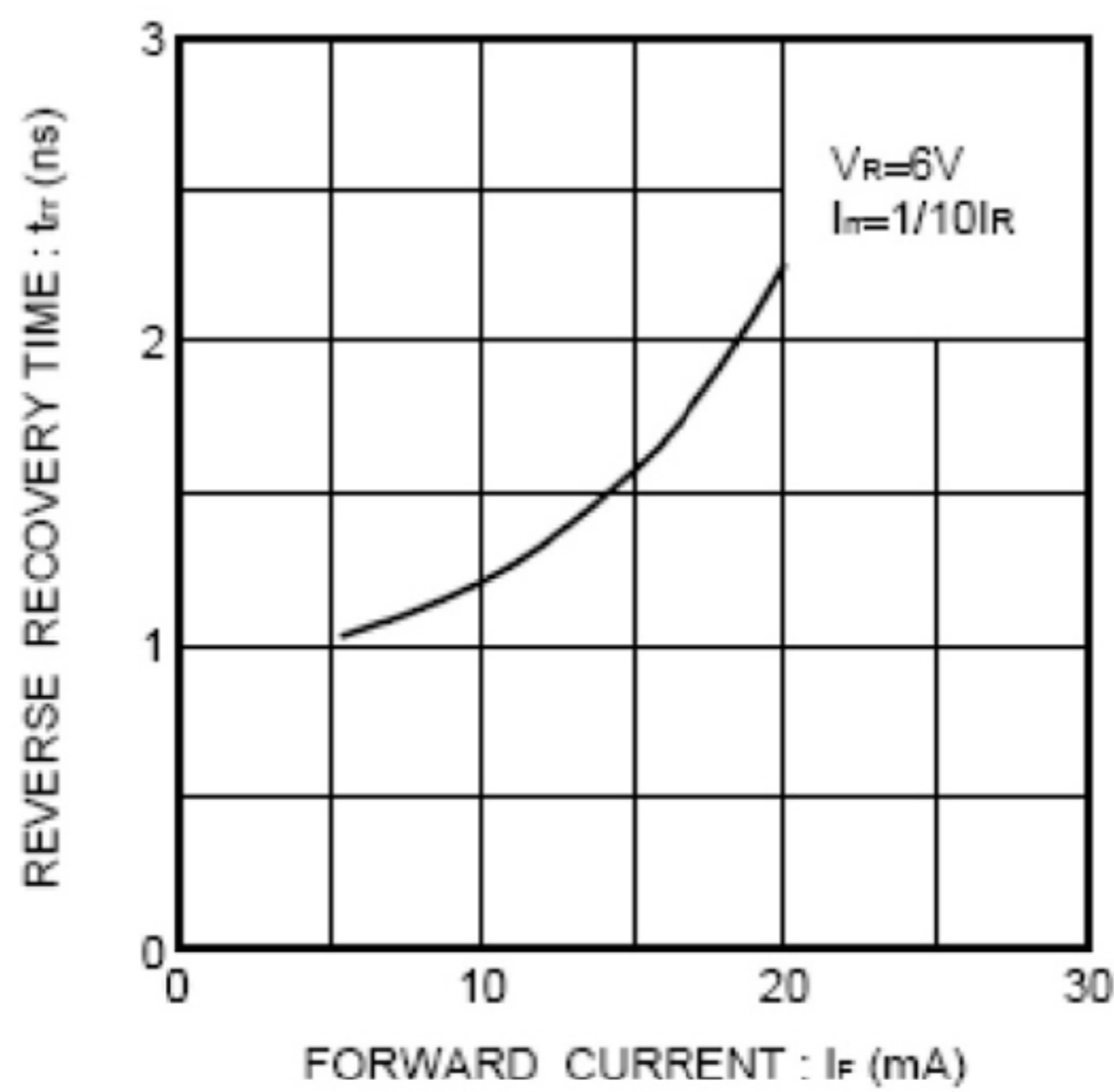
Fig.4 Reverse recovery time characteristics
