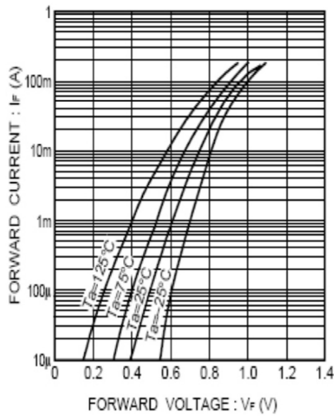
Fig.1 Forward characteristics
