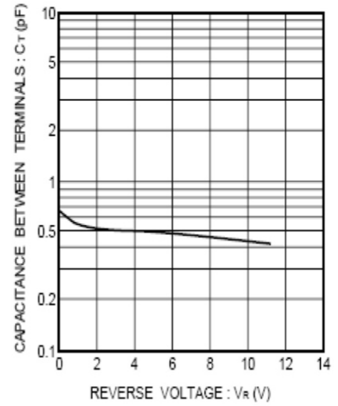
Fig.3 Capacitance between terminals
