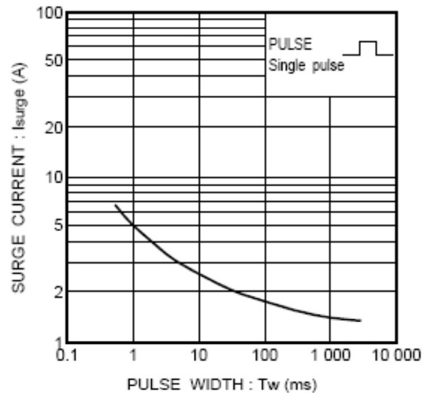
Fig.5 Surge current characteristics
