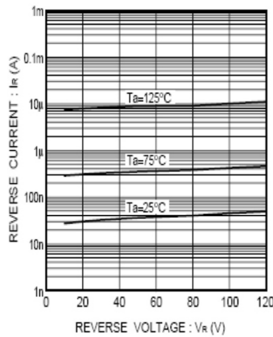
Fig.2 Reverse characteristics
