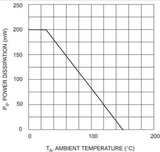
Fig. 5 Power Derating Curve, Total Package
