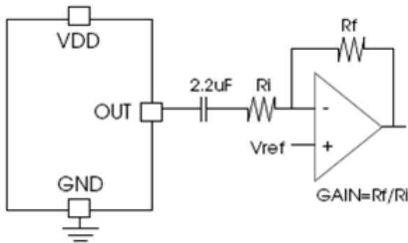
Connect to Audio OPAMP
